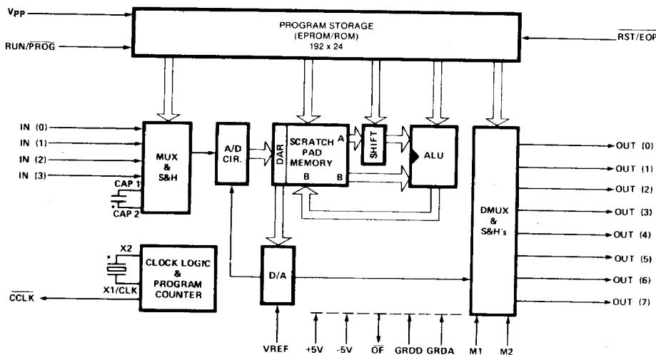
Figure 1. Functional Block Diagram (Run Mode)
