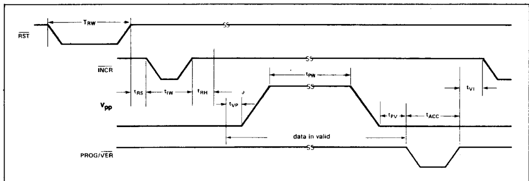
Figure 6. 2920 Program/Verify, 2921 Verify Timing
