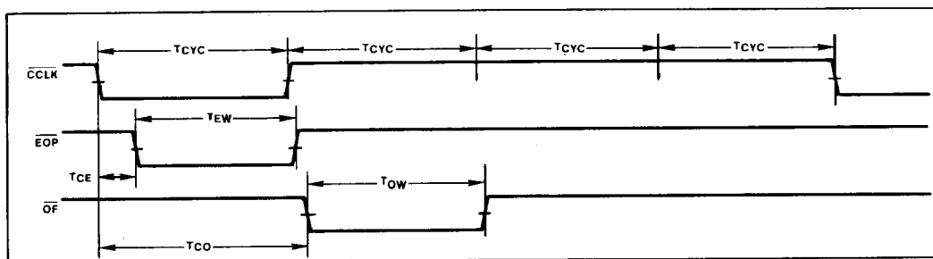
Figure 5. Run Mode Timing
