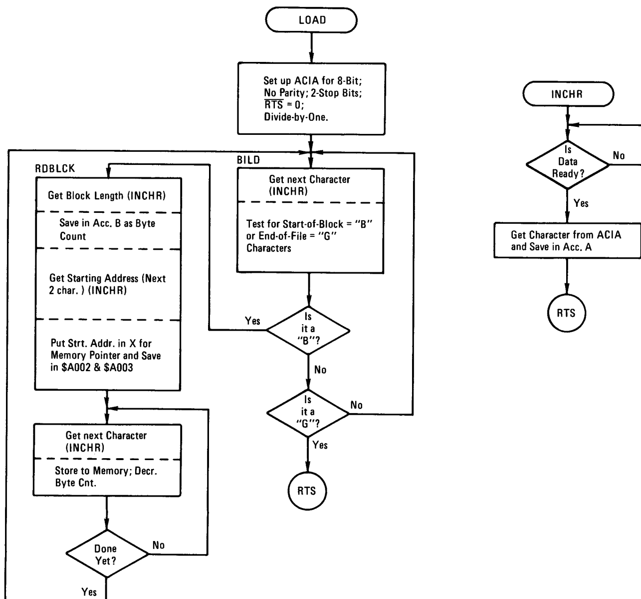
FIGURE 3-7-2. Program Flow for LOAD Function
