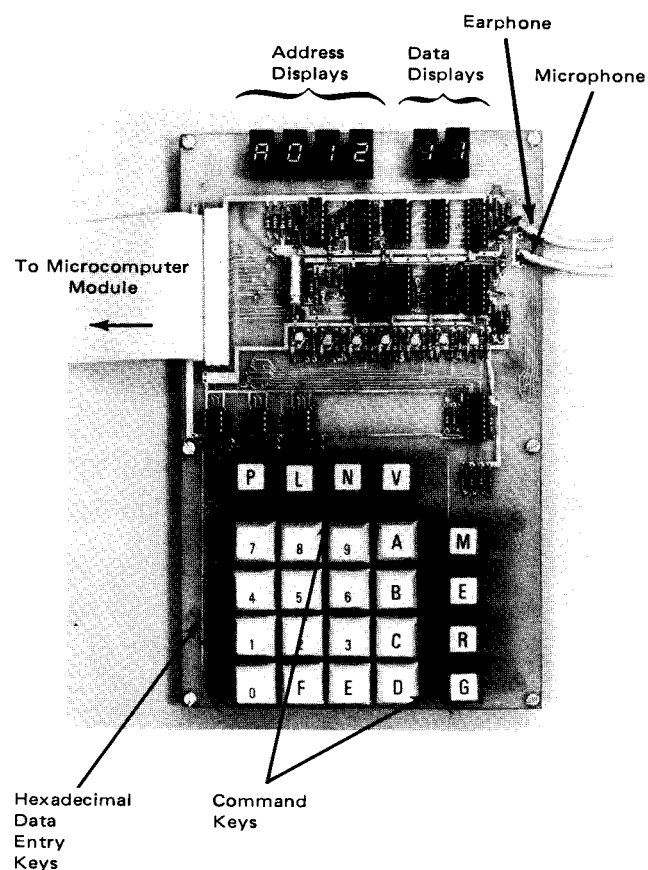
FIGURE 1-1-3b. Keyboard/Display Module
